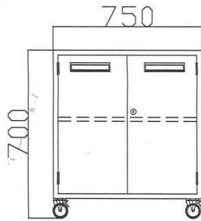
MOVABLE CBINET WITH CASTOR WHEEL QTY-2NOS
